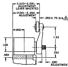
CLOSED MOUNTED ROLLER
