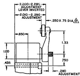
CLOSED MOUNTED ROLLER
