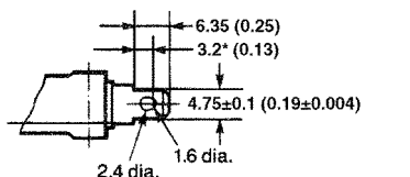
Solder terminal (A) (or quick connect terminals #187 series)
