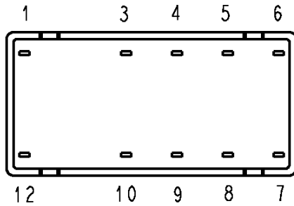
Relay - bottom view
