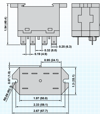
C3 – PANEL/DIN MOUNT (QC/SOLDER TERMINAL)
