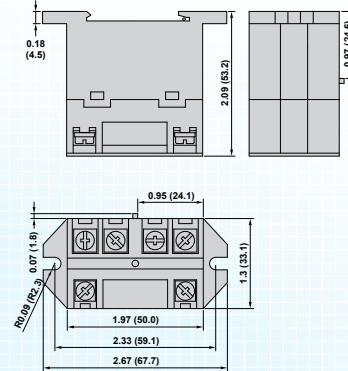
C3 – PANEL/DIN MOUNT (SCREW TERMINAL)
