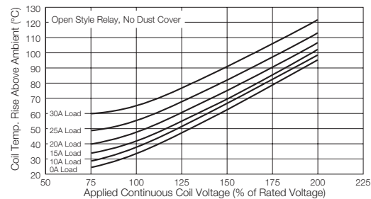
Ambient temperature vs. coil voltage – 1W coil
