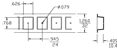
TAPE DETAILS
