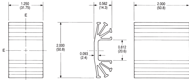
603 SERIES (EXTRUSION PROFILE 1284)
