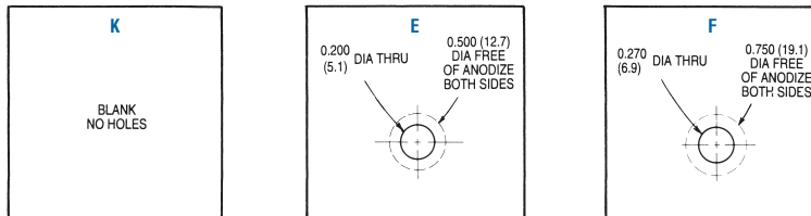
603 SERIES (EXTRUSION PROFILE 1284)
