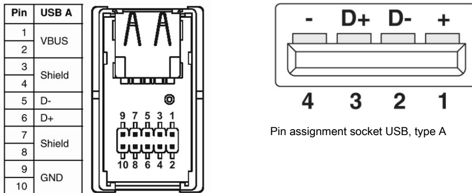
Contact assignment
