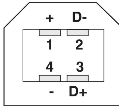
Pin assignment socket USB, type B
