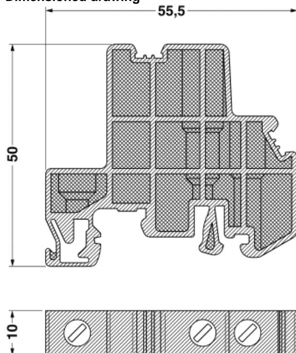
Dimensioned drawing
