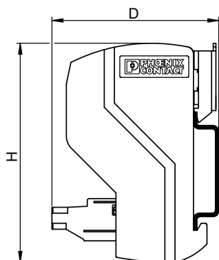
Figure 1 VIP-2/SC/PDM-2/... dimensions
