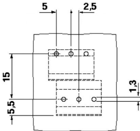
Drilling diagram
