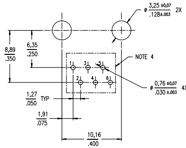
BOARD LAYOUT VIEWED FROM TOP
