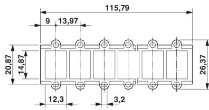
RJ45 panel mounting frame, IP20
