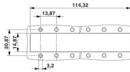
Panel cutout
