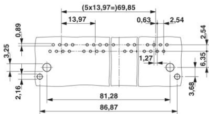
Drilling plan/solder pad geometry
