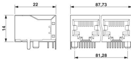
Dimensioned drawing
