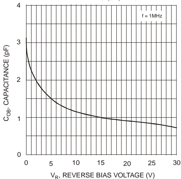
Fig. 4 Output Capacitance
