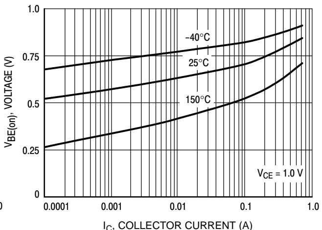
Figure 8. V_{BE(on)} Voltage
