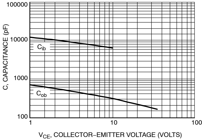
Figure 7. Typical Capacitance
