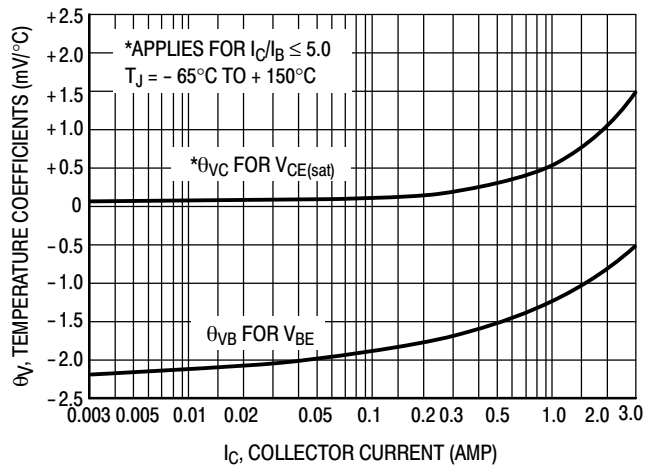
Figure 11. Temperature Coefficients
