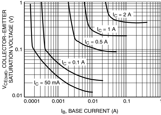
Figure 9. Saturation Region
