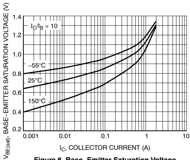
Figure 6. Base-Emitter Saturation Voltage
