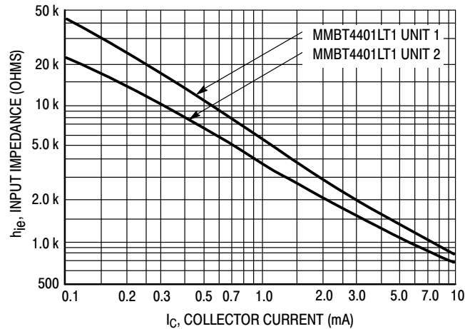
Figure 10. Input Impedance
