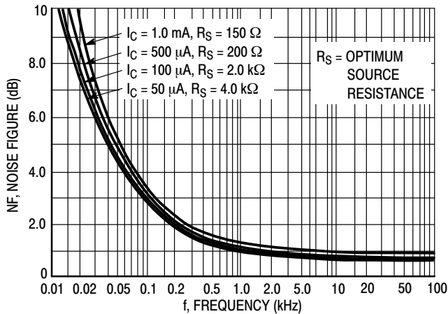
Figure 8. Frequency Effects
