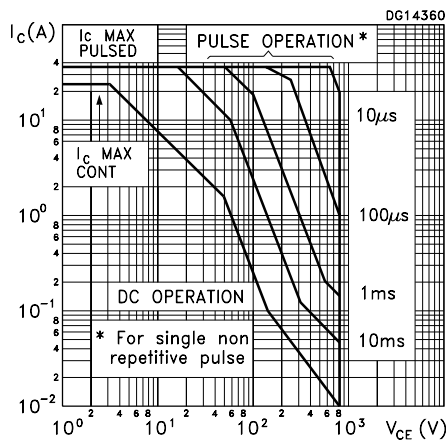
Figure 4: Output Characteristics
