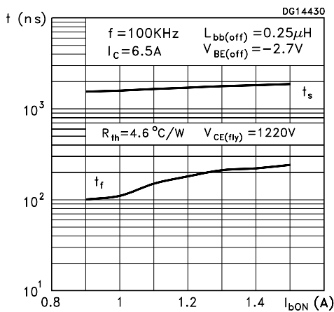
Figure 11: Inductive Load Switching Time
