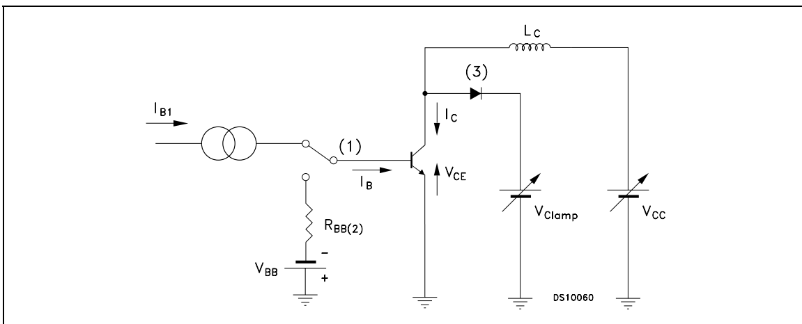
Figure 16: Reverse Biased Safe Operating Area Test Circuit
