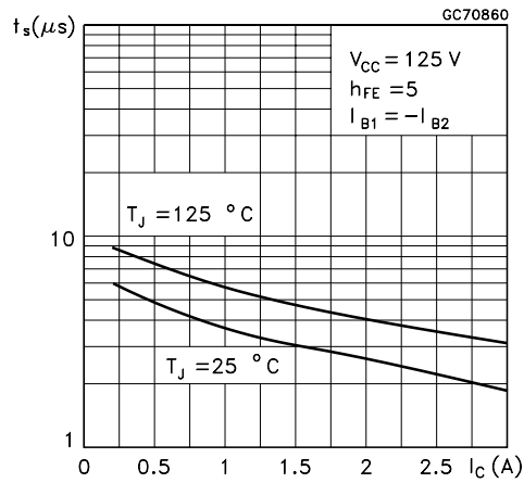
Figure 13: Resistive Load Storage Time
