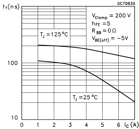
Figure 10: Resistive Load Fall Time
