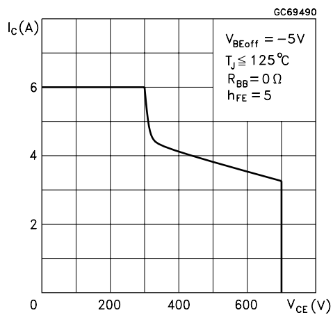
Figure 11: Reverse Biased Operating Area
