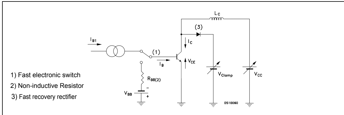
Figure 14: Inductive Load Switching Test Circuit
