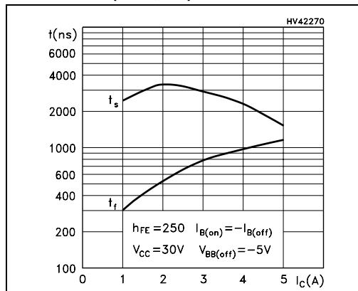
Figure 14. Resistive load switching time (NPN, off)
