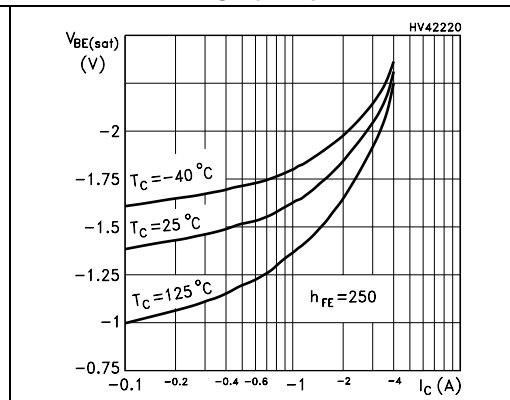
Figure 9. Base-emitter saturation voltage (PNP)
