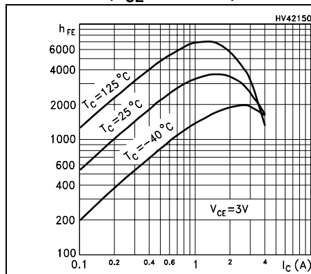
Figure 2. DC current gain ( V_{\text{CE}} = 3\text{ V NPN} )
