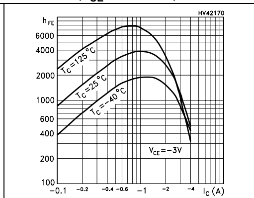
Figure 3. DC current gain ( V_{\text{CE}} = -3\text{ V PNP} )
