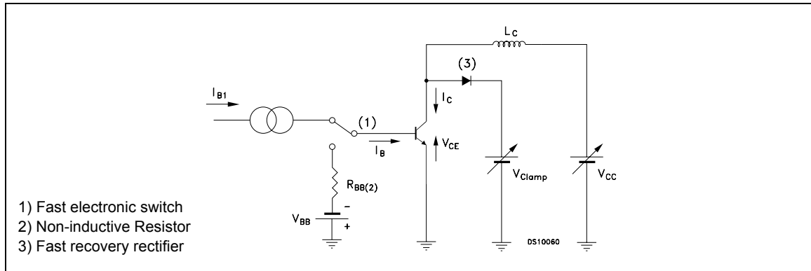
Figure 3: Inductive Load Switching Test Circuit
