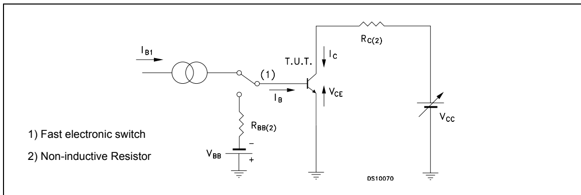
Figure 4: Resistive Load Switching Test Circuit
