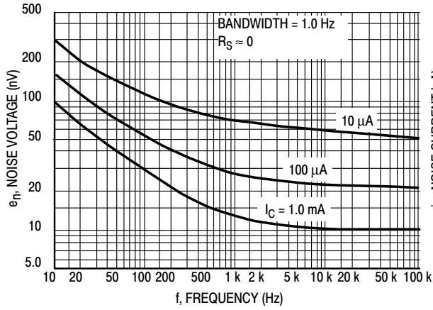
Figure 2. Noise Voltage
