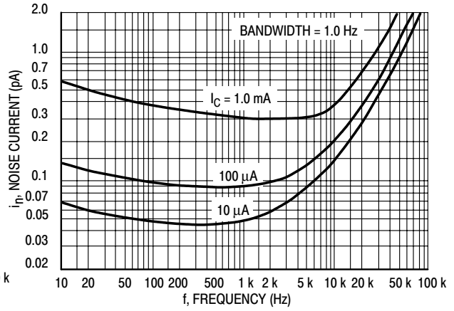
Figure 3. Noise Current
