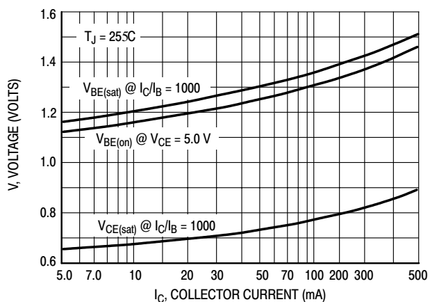
Figure 10. "On" Voltages
