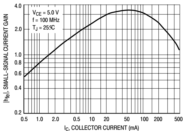
Figure 7. High Frequency Current Gain
