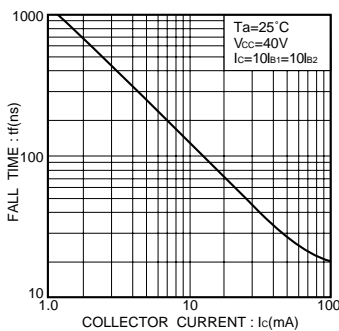
Fig.12 Fall time vs. collector current
