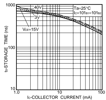
Fig.11 Storage time vs. collector current
