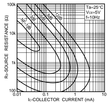
Fig.19 Noise characteristics (I)
