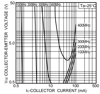
Fig.14 Gain bandwidth product
