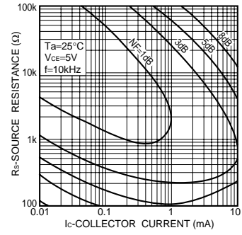
Fig.22 Noise characteristics (IV)
