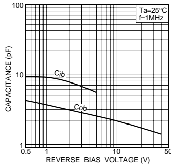
Fig.13 Input/output capacitance vs. voltage
