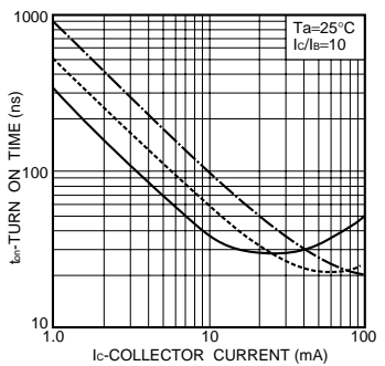
Fig.9 Turn-on time vs. collector current
