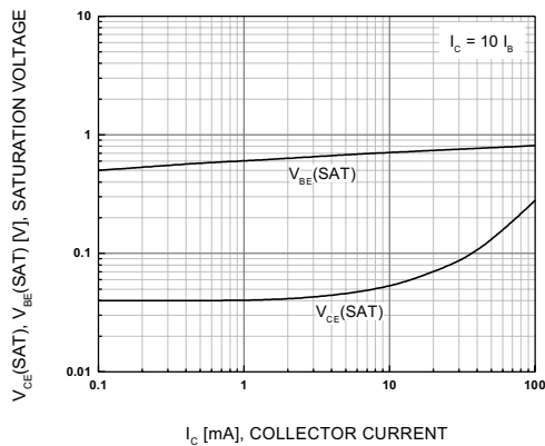
Figure 5. Saturation Voltage
