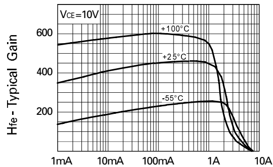
I_C -Collector Current
