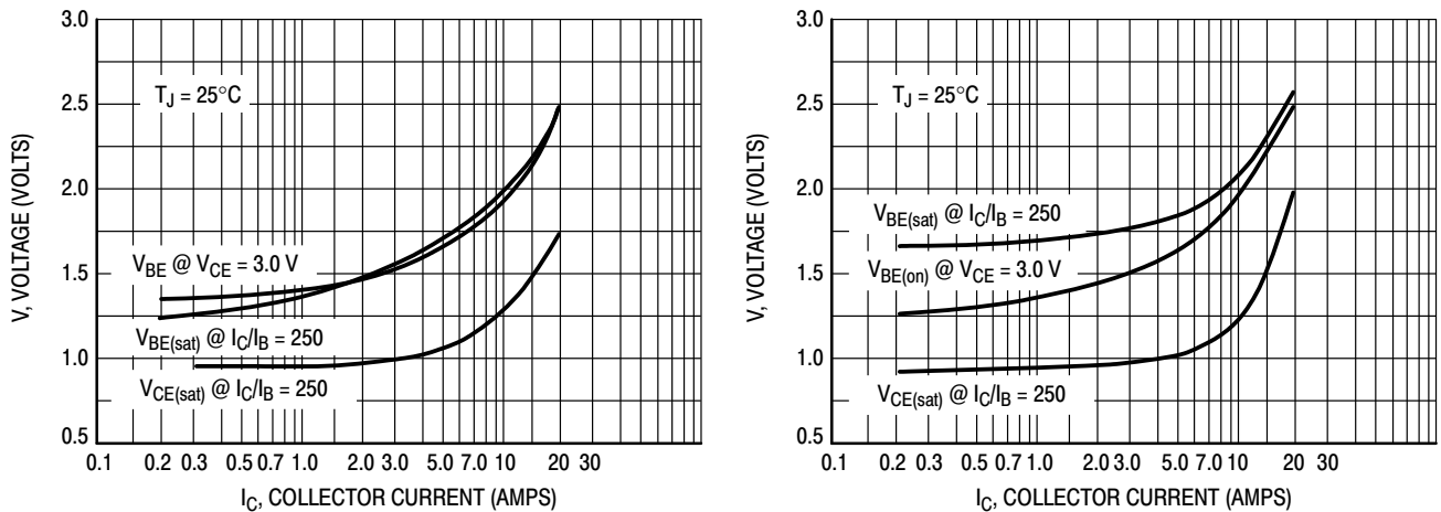
Figure 9. "On" Voltages
