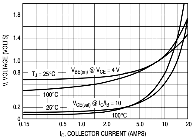
Figure 5. "On" Voltage
