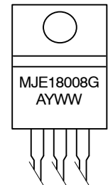
TO-220AB CASE 221A-09 STYLE 1
