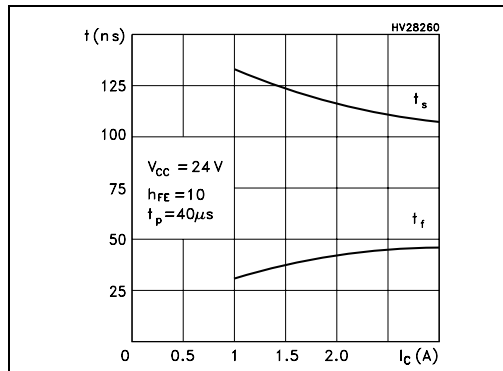
Figure 6. Switching times on resistive load
