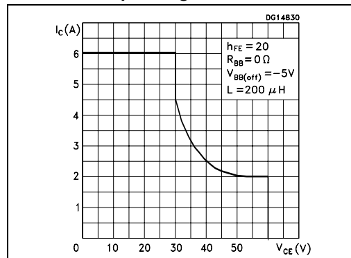
Figure 8. Reverse biased safe operating area
