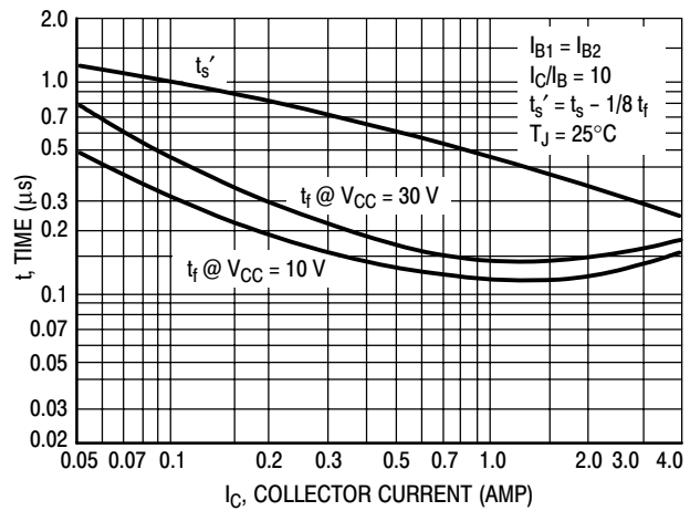
Figure 10. Turn-Off Time
