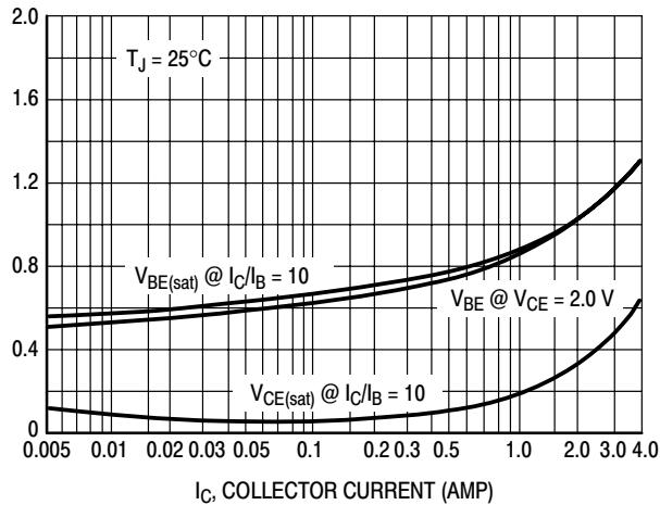
Figure 3. "On" Voltages
