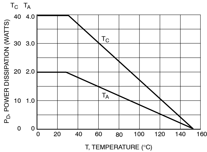
Figure 1. Power Derating
