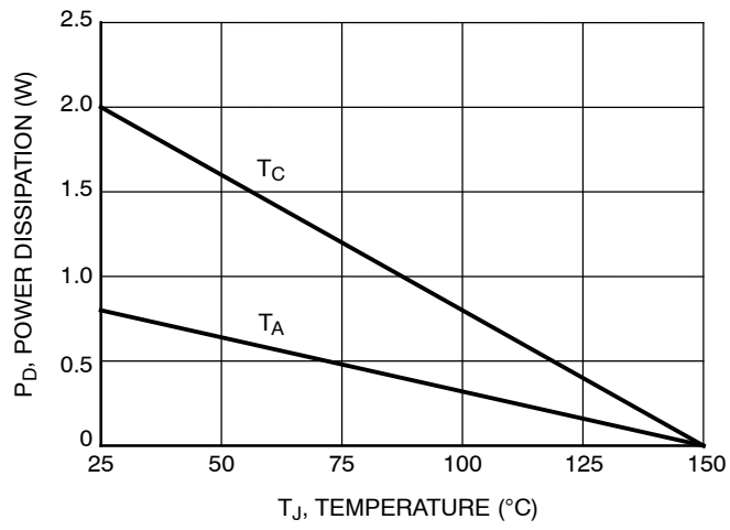
Figure 1. Power Derating
