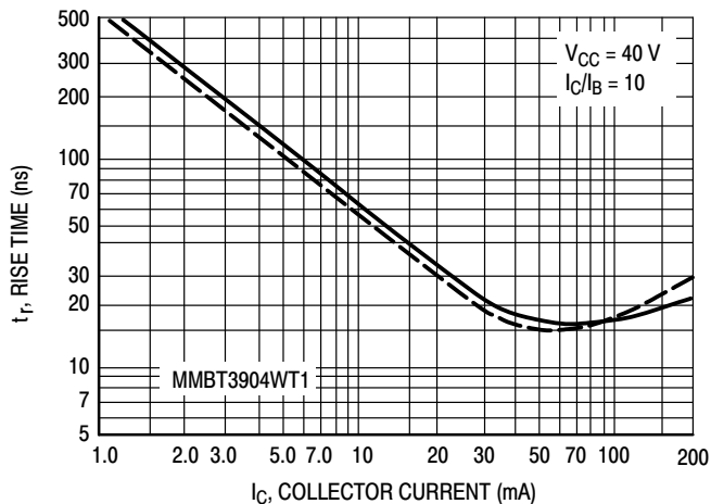
Figure 4. Rise Time
