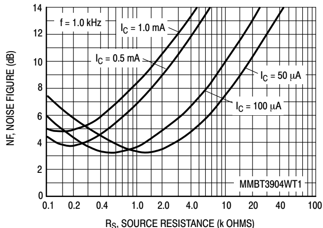
Figure 8. Noise Figure
