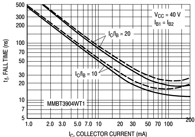
Figure 6. Fall Time
