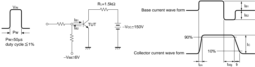
Fig.10 Switching time measurement circuit
