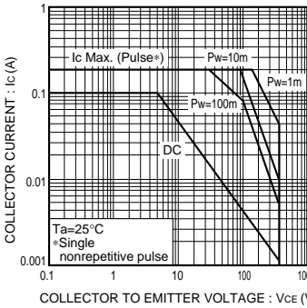
Fig.9 Safe operating area
