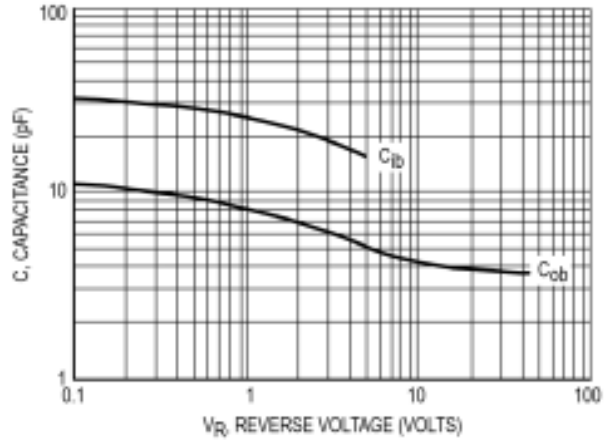
Capacitances
