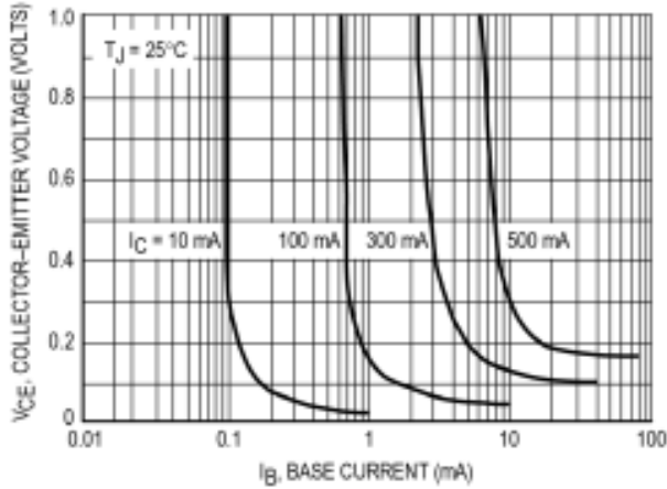
Saturation Region
