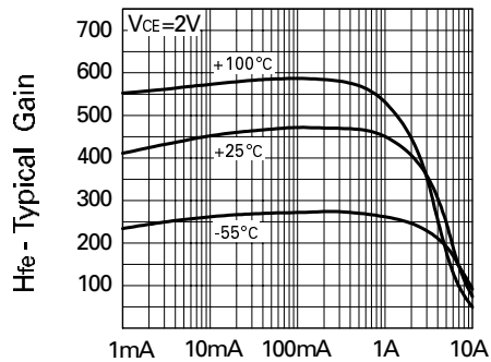
IC-Collector Current h_{FE} v I_C
