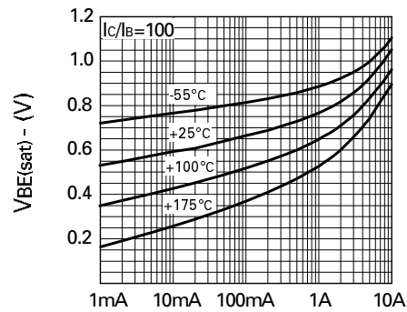
IC-Collector Current V_{BE(sat)} v I_C
