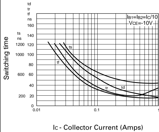
Switching Speeds
