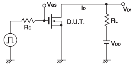
Fig. 16 Switching time measurement circuit
