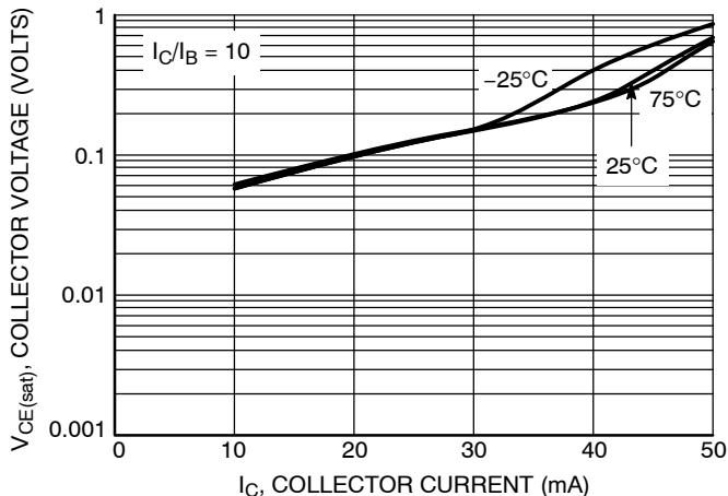
Figure 133. V_{CE(sat)} versus I_C
