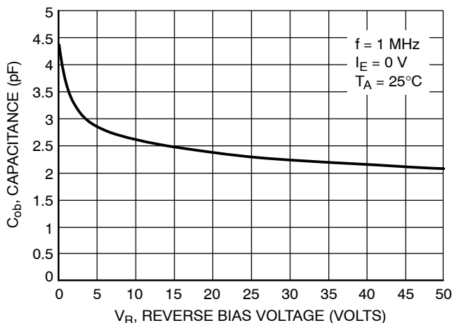
Figure 135. Output Capacitance
