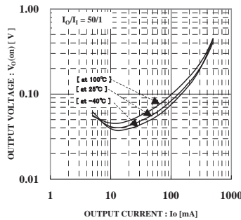
Fig.5 Output voltage vs. output current II
