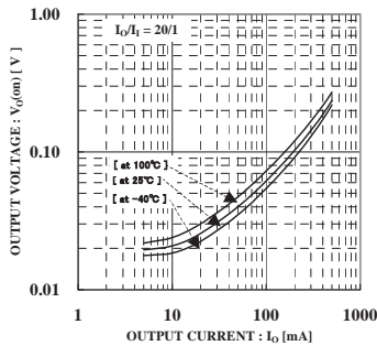
Fig.4 Output voltage vs. output current I
