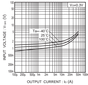
Fig.8 Input voltage vs. output current (ON characteristics)
