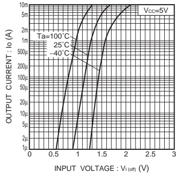
Fig.7 Output current vs. input voltage (OFF characteristics)
