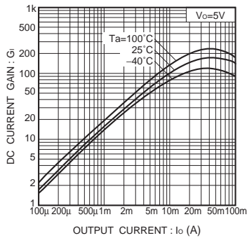
Fig.10 DC current gain vs. output current
