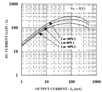
Fig.6 DC current gain vs. output current
