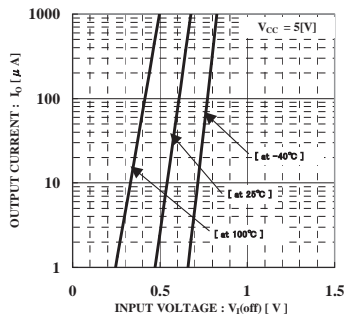
Fig.1 Output current vs. input voltage (OFF characteristics)
