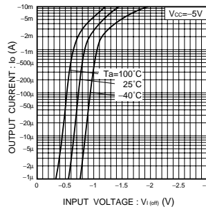
Fig.2 Output current vs. input voltage (OFF characteristics)
