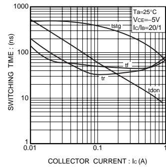
Fig.6 Switching time
