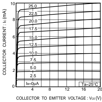
Fig.8 Ground emitter output characteristics
