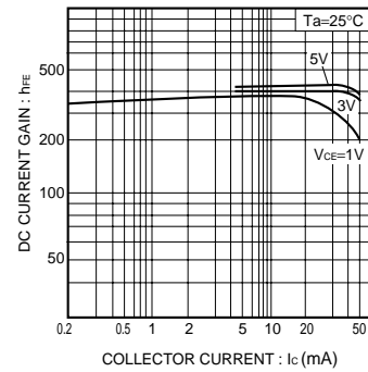
Fig.10 DC current gain vs. collector current
