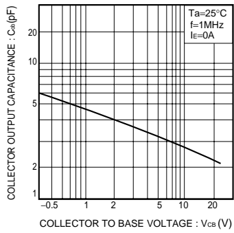
Fig.14 Collector output capacitance vs. collector-base voltage
