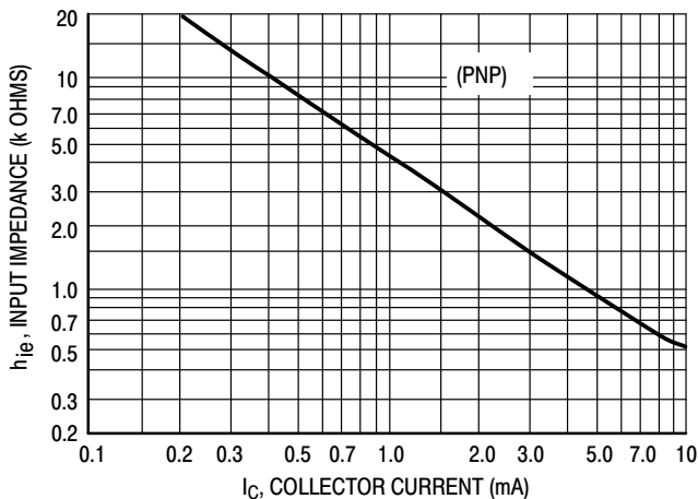
Figure 27. Input Impedance
