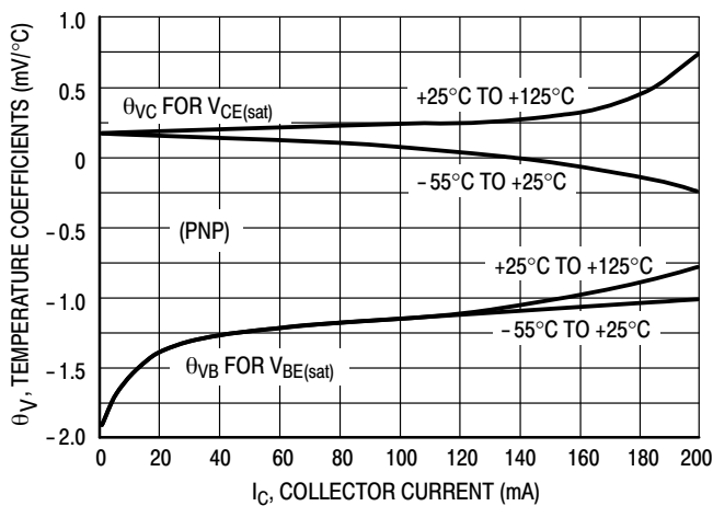
Figure 32. Temperature Coefficients
